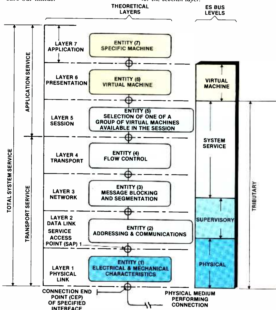
Figure 3. Communications theory breaks the remote-control process into seven layers. The ES bus concept redivides layers into four levels. Because the specific machine is a manufacturer concern that is resolved at the virtual machine level, no specification is made for the seventh layer.
